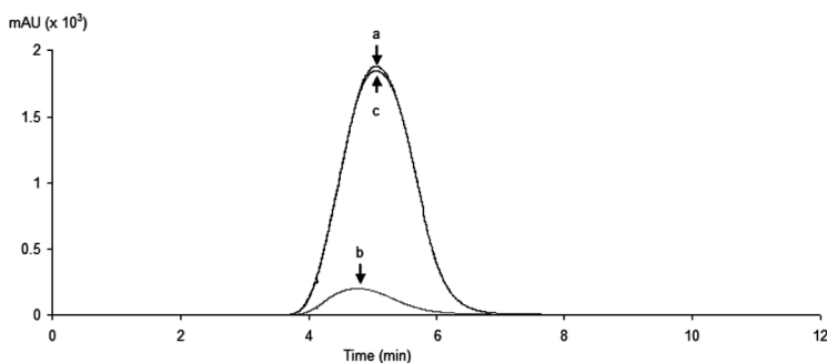
Figure 3. Screening of a cholinesterase inhibitor on a BuChE-IMER. Chromatograms showing subsequent injections to a BuChE-IMER of butyrylthiocholine at saturating substrate concentration (a), with 1 mM tacrine inhibitor (b), and again with butyrylthiocholine at saturating substrate concentration (c).
